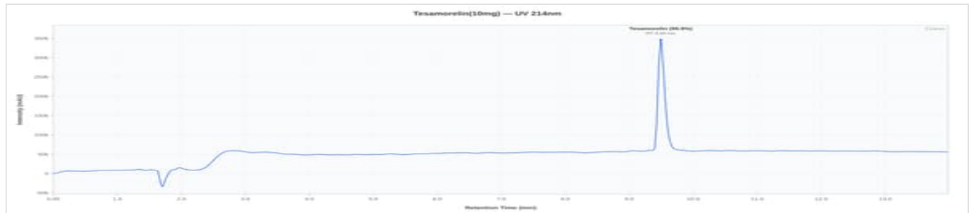
Tesamorelin 10mg - LOT-2026-08: UV Chromatogram
