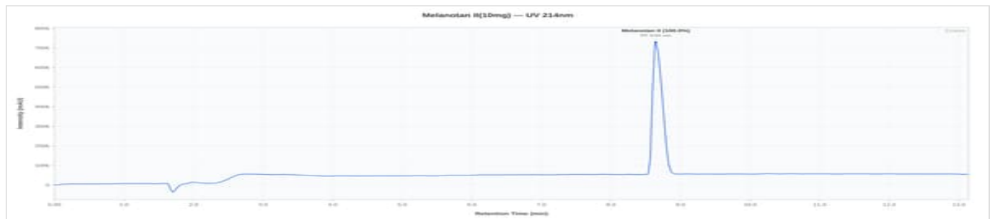
MT-2 10mg - LOT-2026-08: UV Chromatogram
