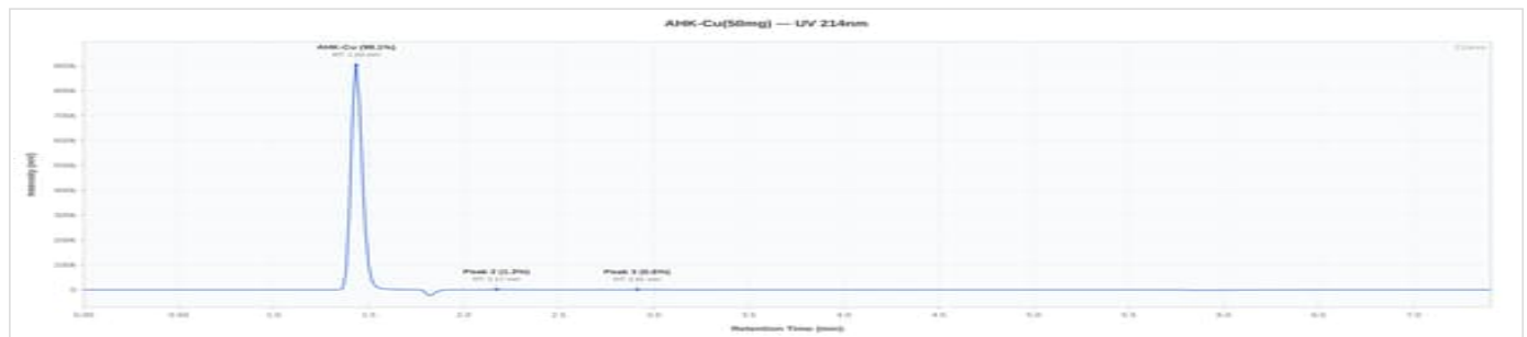
AHK-Cu 50mg - LOT-2026-08: UV Chromatogram
